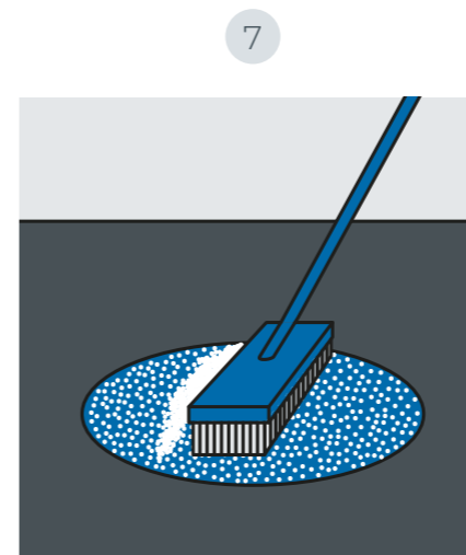
Clean the marking with a broom and use a sharp object to check that it is securely adhered. It can be driven over after just a few minutes.
